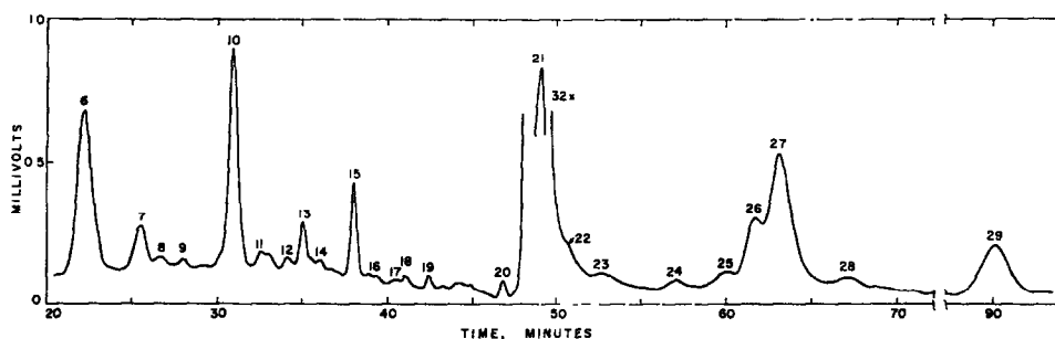
FIG. 1. VOLATILE BASES OF CIGAR SMOKE.
